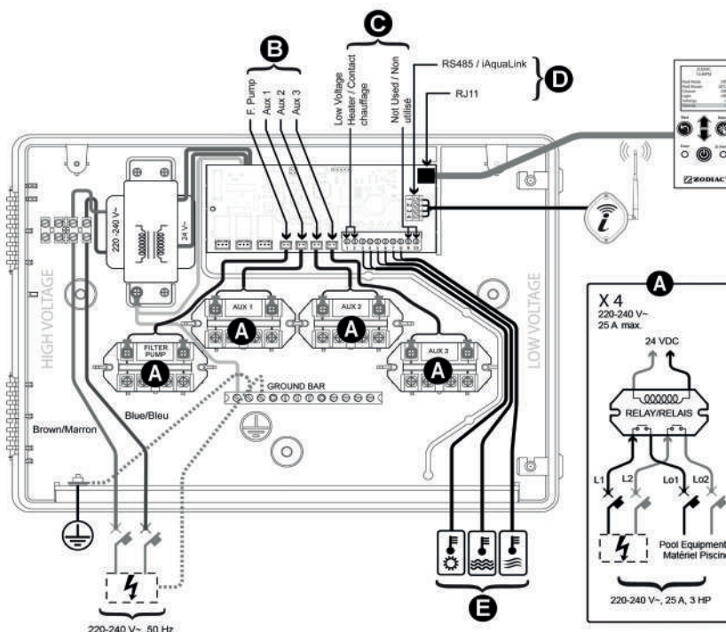
Diagram of standard connections on AquaLink® TRi
