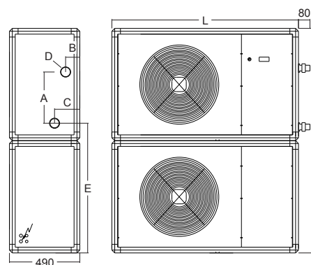
Z600 Silent TD9 and TD12
