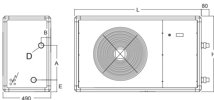
Z600 Silent MD5 MD7 and TD7
