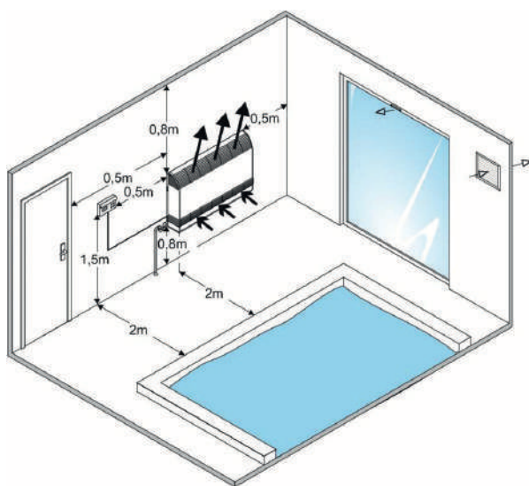
Example of an installation with a SIROCCO Free-discharge console
