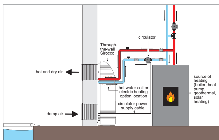
Installation of an appliance with the hot water coil option.
