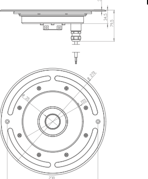
I1265 CIRCULAR Ø200 DRY FOUNTAIN
