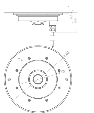
I1264 CIRCULAR Ø200 FLAT MOUNTING
