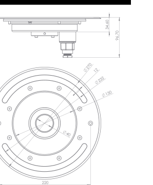
I1288 CIRCULAR Ø200 DRY FOUNTAIN Ø40MM
