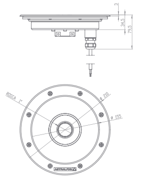
I1262 CIRCULAR Ø200 1" THREAD
