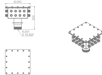
CABLE INLET FITTING BOX 66607
