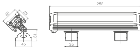
11279 LINEAR ADJUSTABLE PROJECTOR
