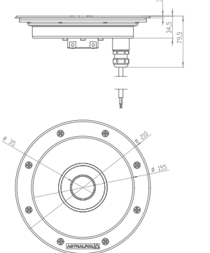
I1263 CIRCULAR Ø200 NO THREAD
