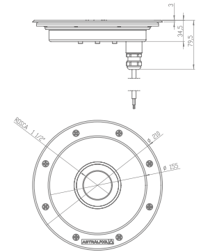
I1261 CIRCULAR Ø200 1" 1/2 THREAD
