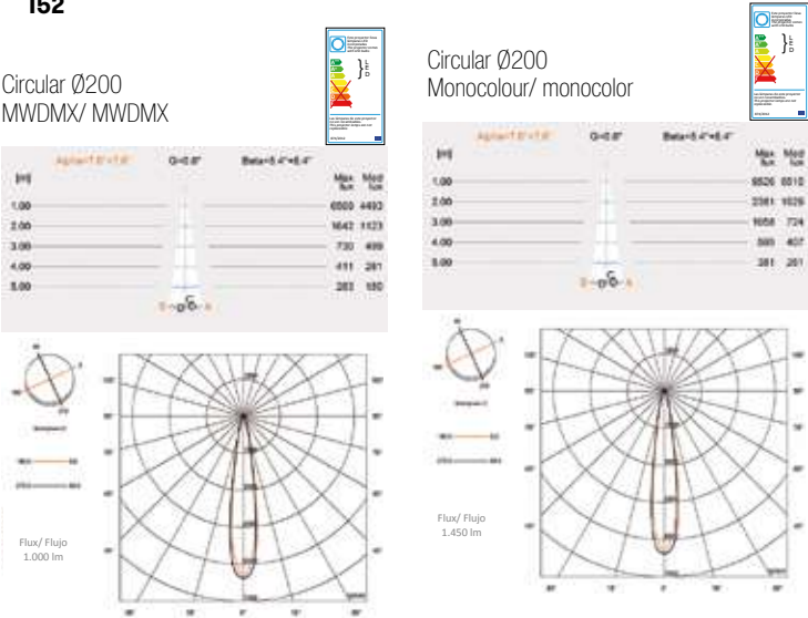
I1263 CIRCULAR Ø200 NO THREAD
