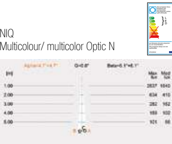
I1245 NIQ RECESSED PROJECTOR (PVC NICHE)
